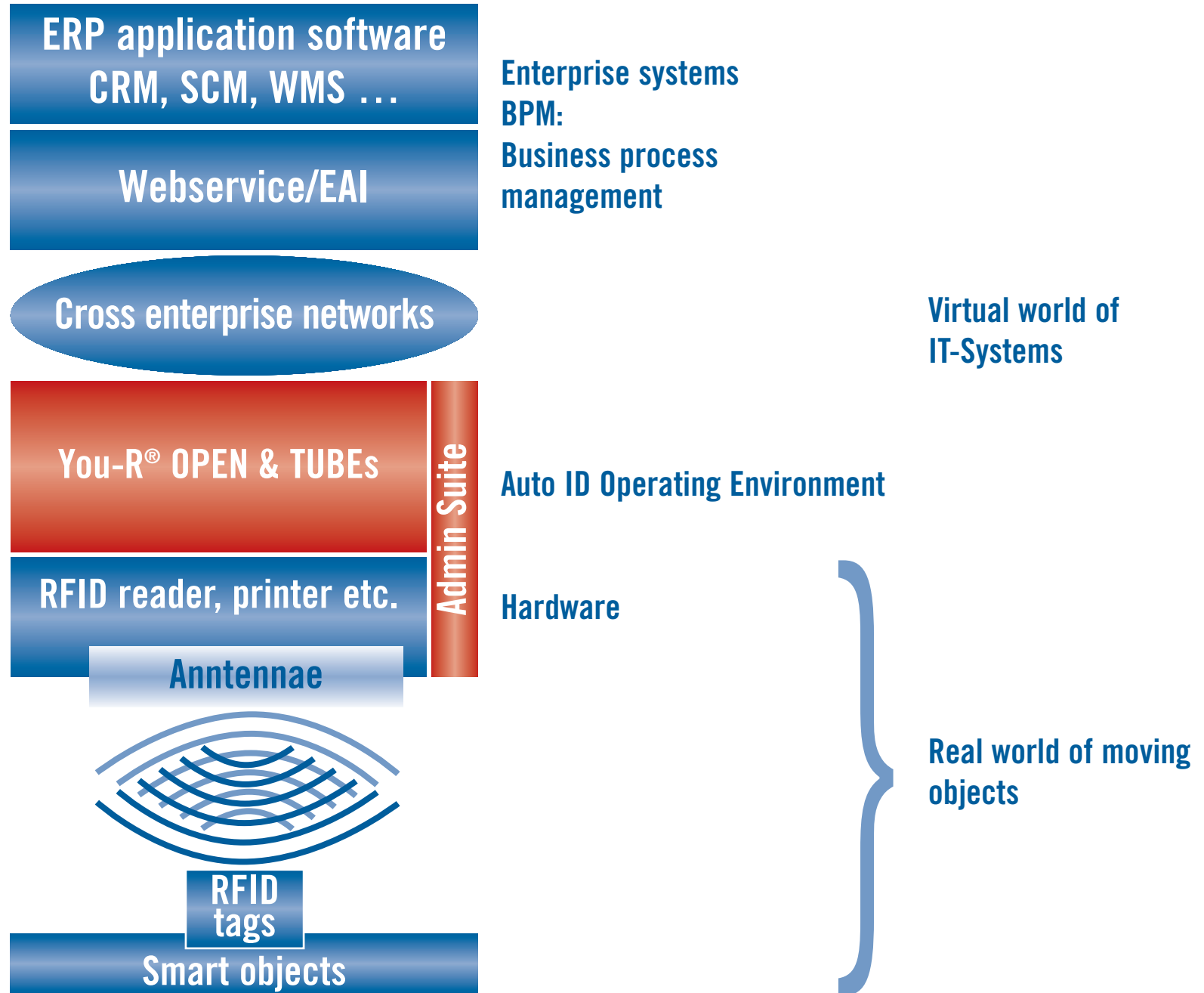
Auto ID Operating Environment embedded in an Enterprise Systems Architecture
